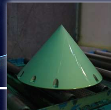
Fluorescent Penetrant Inspection (FPI)
